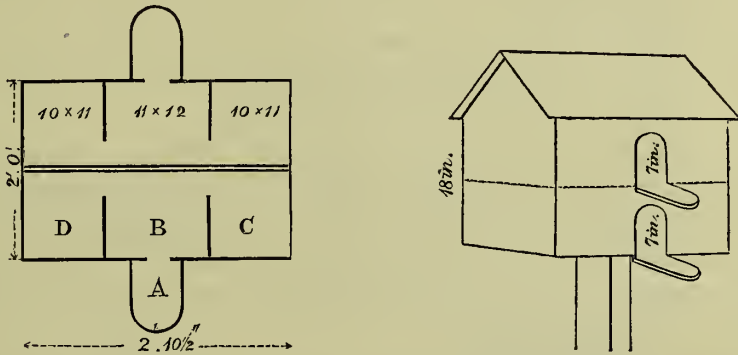
FIG. VI.—PLAN AND ELEVATION OF A TWO-STORIED POLE PIGEON-HOUSE.
